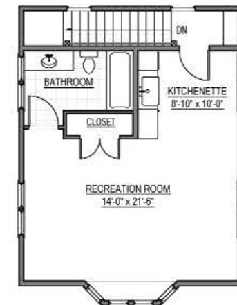
GARAGE F SECOND FLOOR GARAGE PLAN SCALE: 1/8" = 1'-0"
