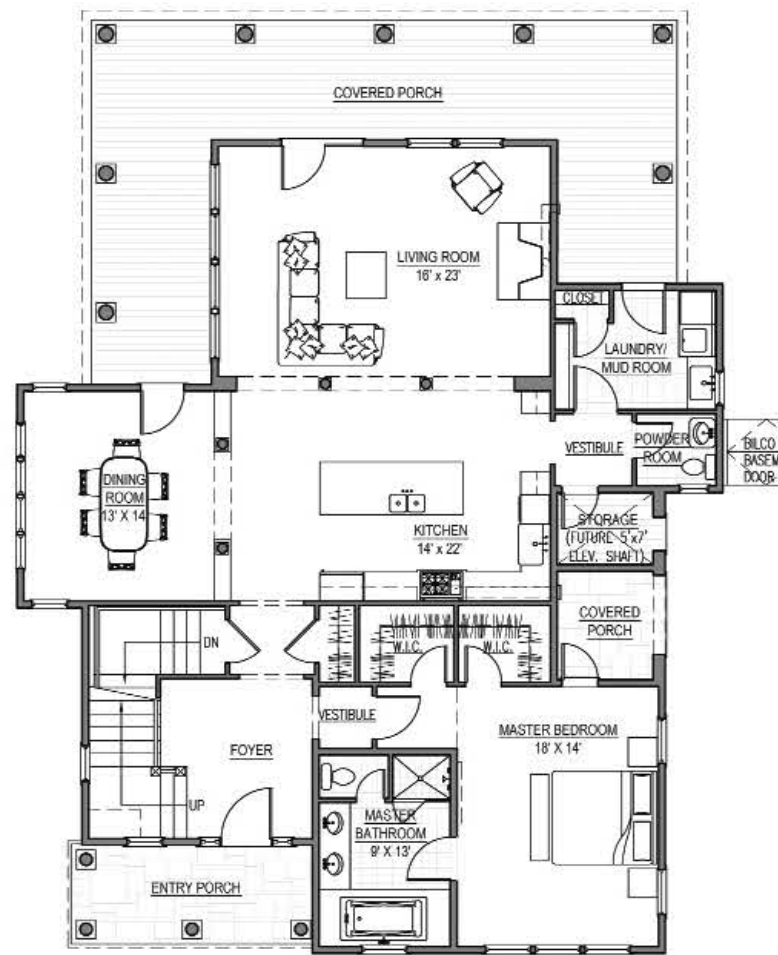
HOUSE D FIRST FLOOR PLAN - 2,013 G.S.F. SCALE: 1/8" = 1'-0"
