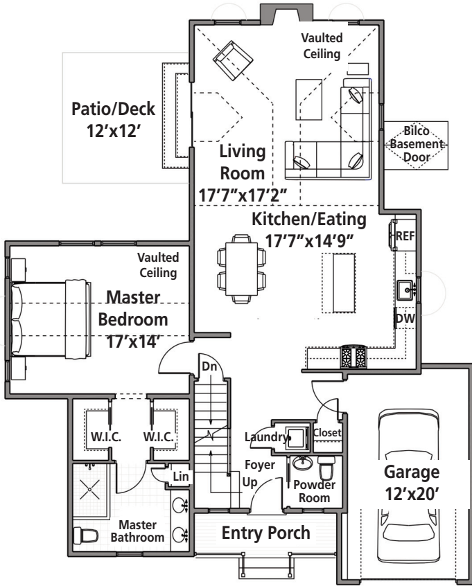
FIRST FLOOR PLAN - 1,315 G.S.F.
