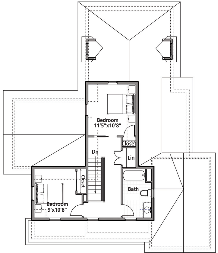
SECOND FLOOR PLAN - 464 G.S.F.
